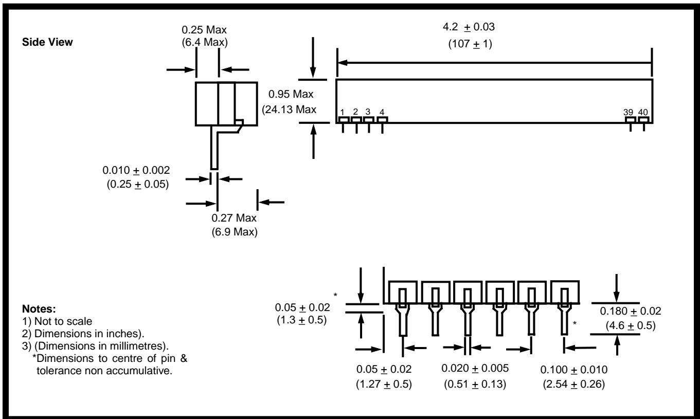
Figure 5 - Mechanical Data
